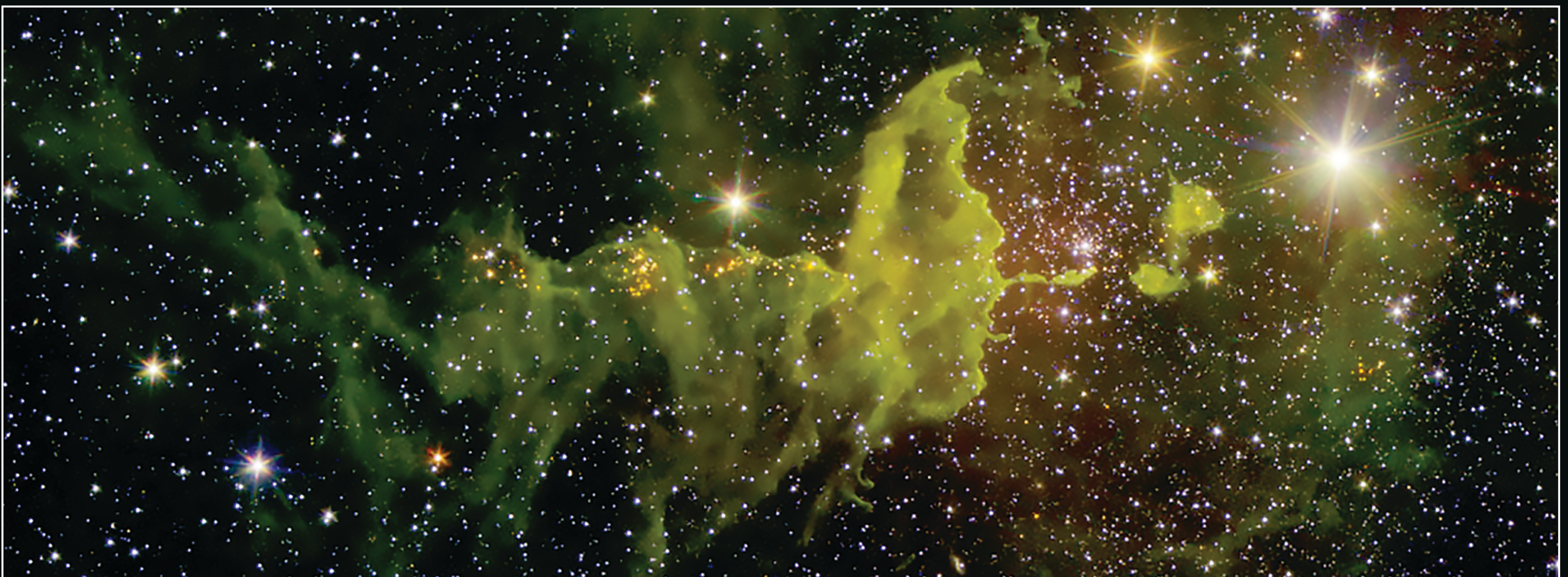
Spider Nebula
