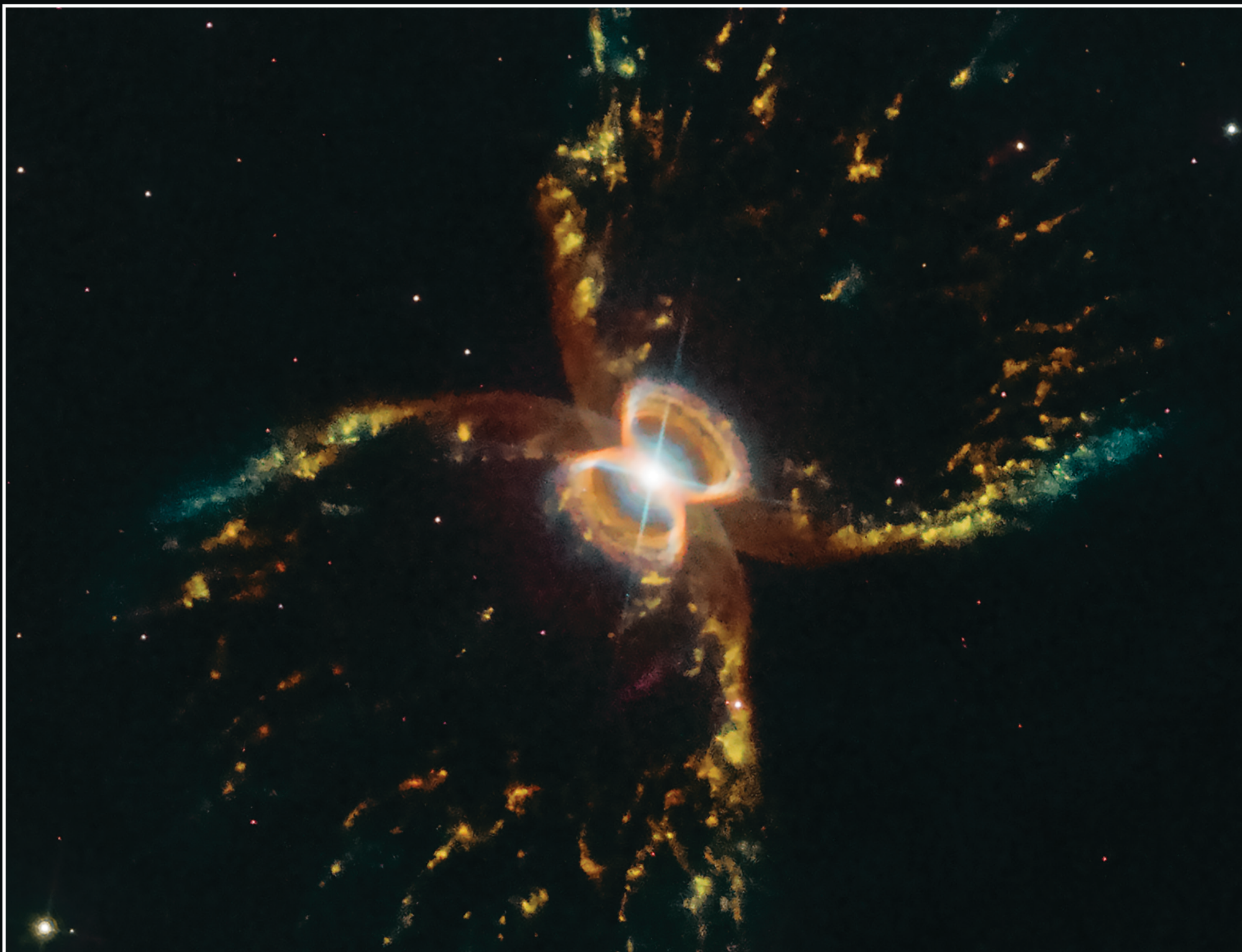
Southern Crab Nebula
