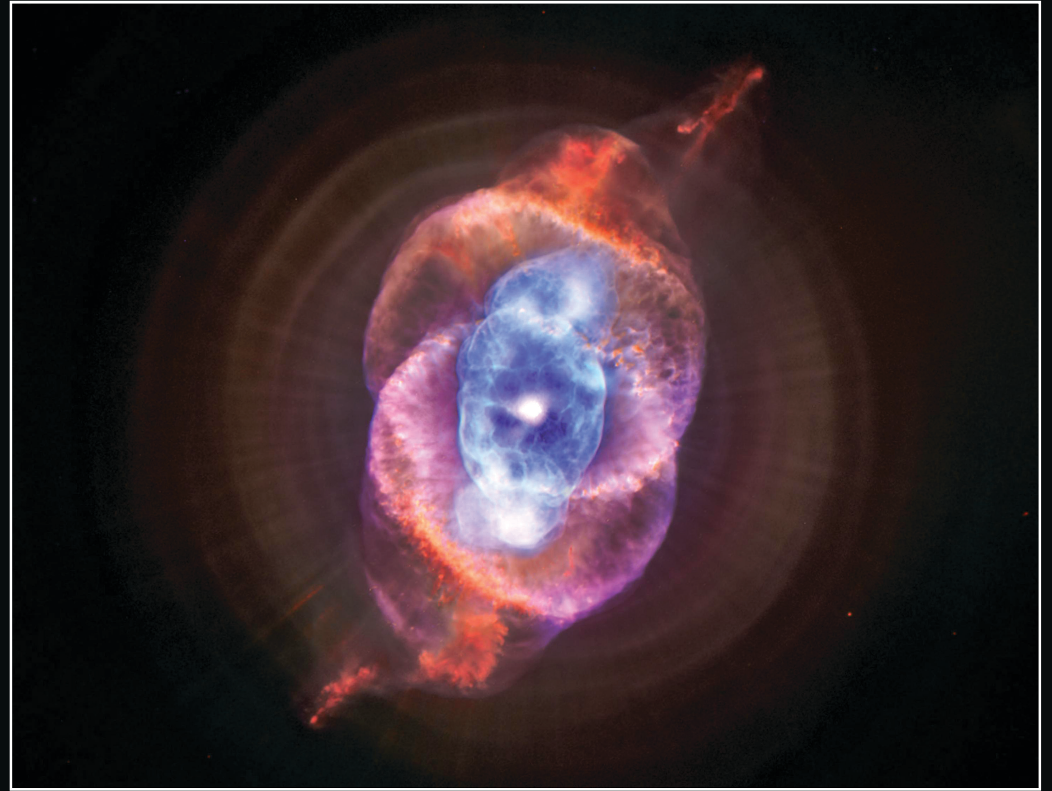
Cat's Eye Nebula
